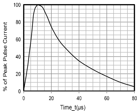
8 X 20 \mu s Pulse Waveform
